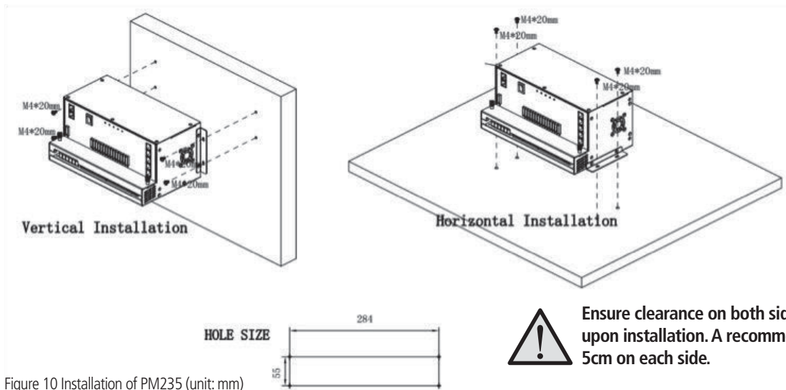
Figure 10 Installation of PM235 (unit: mm)
